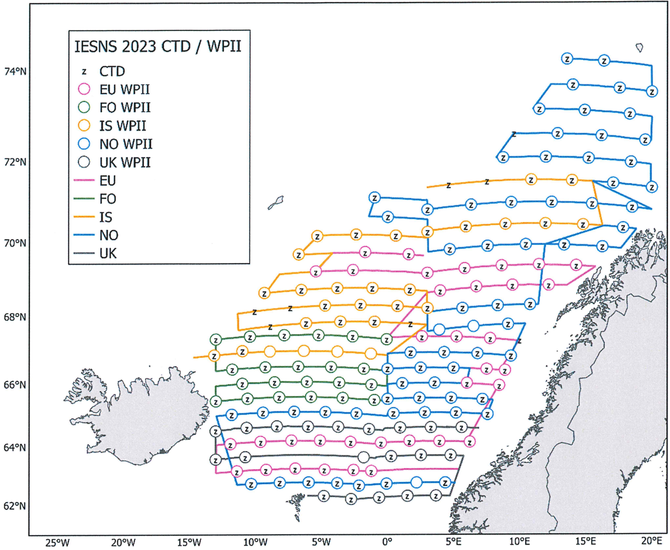
Fig. 1: Survey area for the IESNS with acoustic transects and CTD and plankton stations as carried out in 2023. The 2024 survey will cover the same area with similar spacing between transects and hydrographic stations. At the time of this application the transects have not yet been assigned to the participants of the 2024 survey and it is therefore not possible to indicate yet which of these will be covered by Dana in the 2024 survey.
